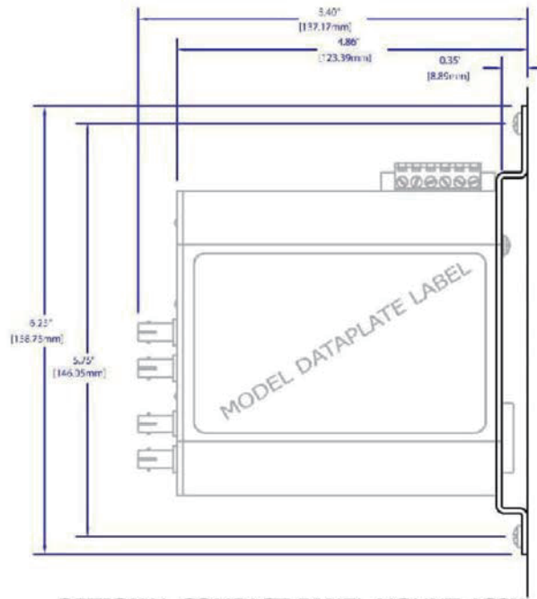
OPTIONAL COMPACT PANEL MOUNT ASSY. ( P/N: CPMA-1 )
