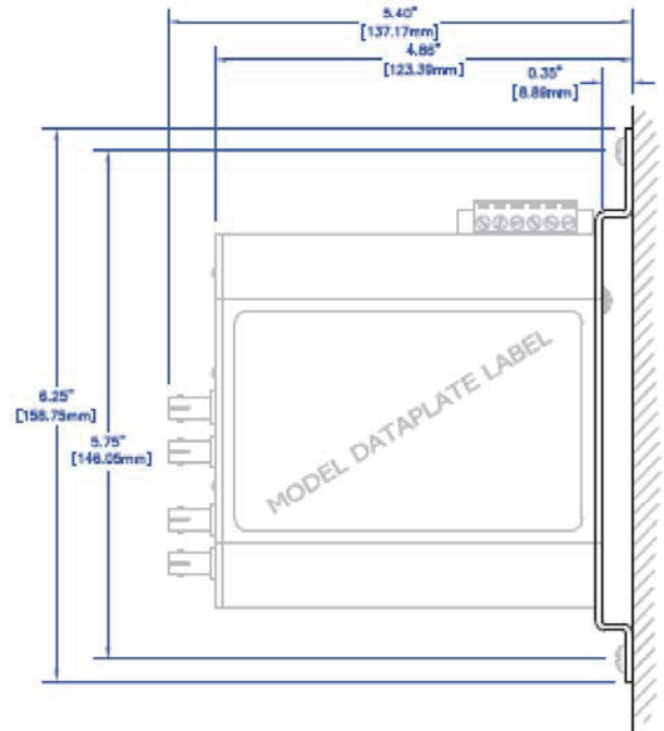
OPTIONAL COMPACT PANEL MOUNT ASSY, ( P/N: CPMA-1 )
