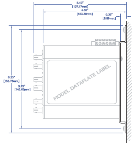
OPTIONAL COMPACT PANEL MOUNT ASSY. ( P/N: CPMA-1 )
